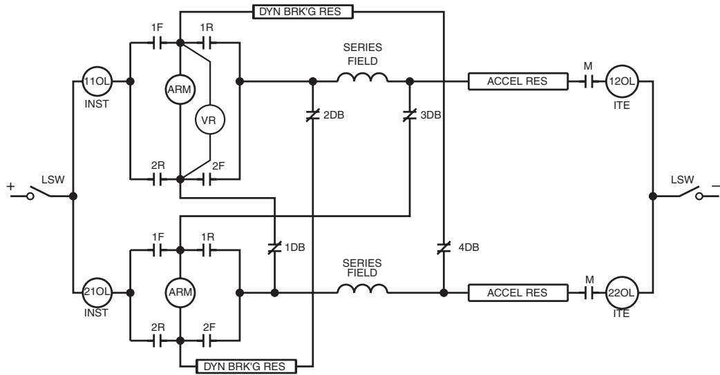
Emergency Dynamic Braking for 2 Motors in Parallel
