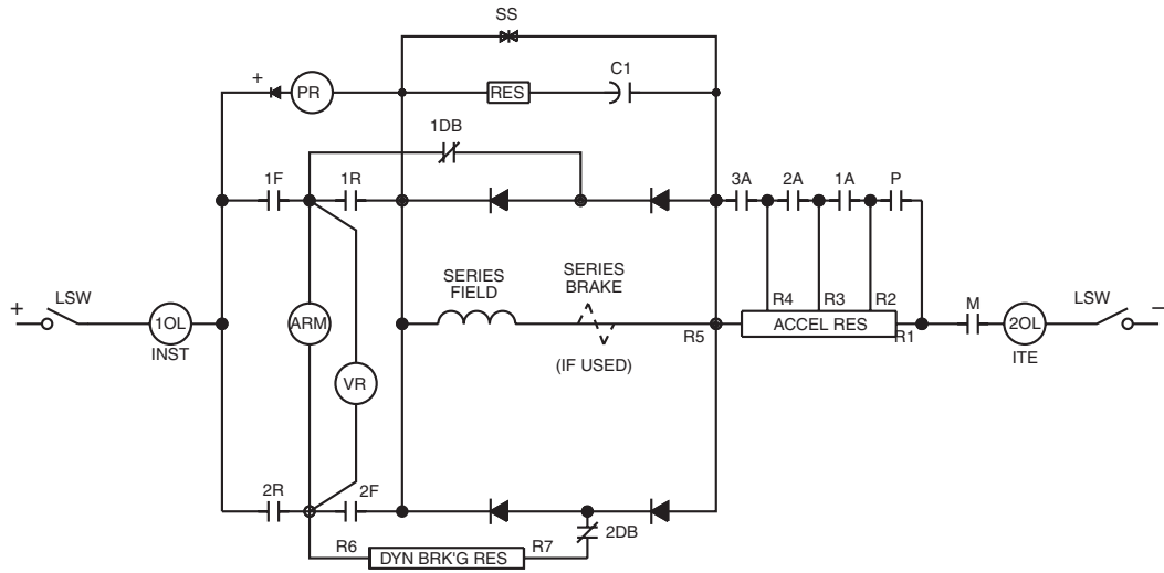
Emergency Dynamic Braking for Single Motor
